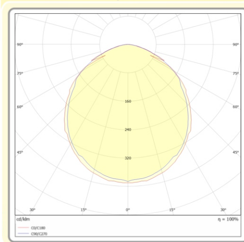
Diagramma polare ECOTEK Polar diagram ECOTEK
