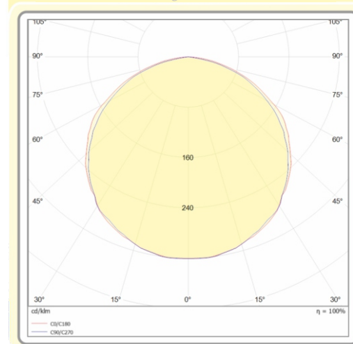
Diagramma polare MINIKEY Polar diagram MINIKEY
